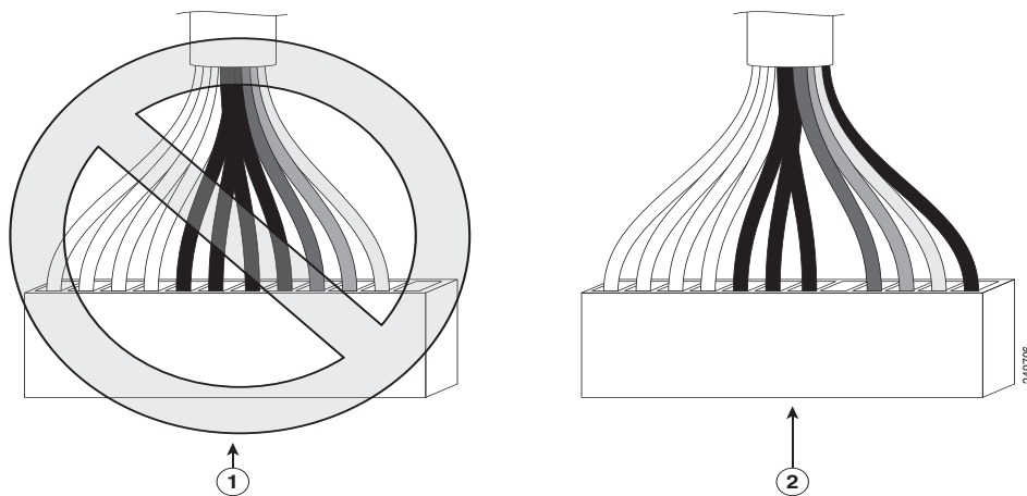
Figure 1 AC Cable to Use When Installing PoE in Cisco 1941 ISRs
