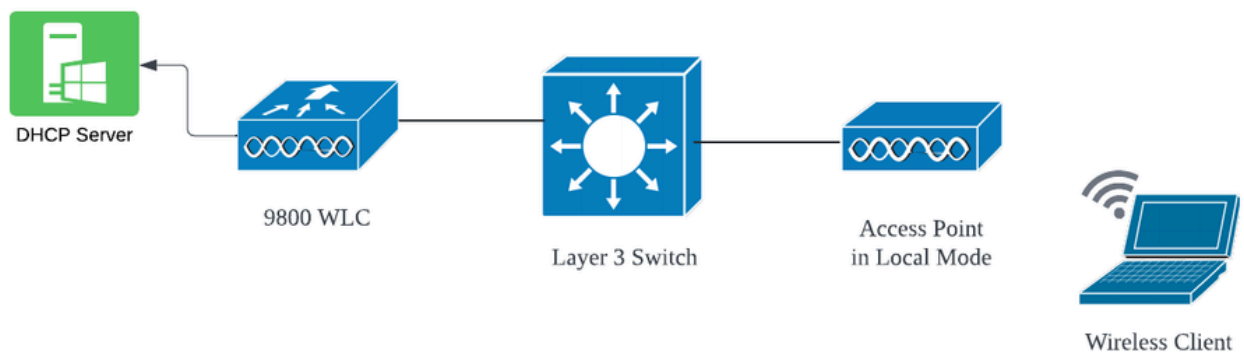
Network Topology : Local Mode AP
