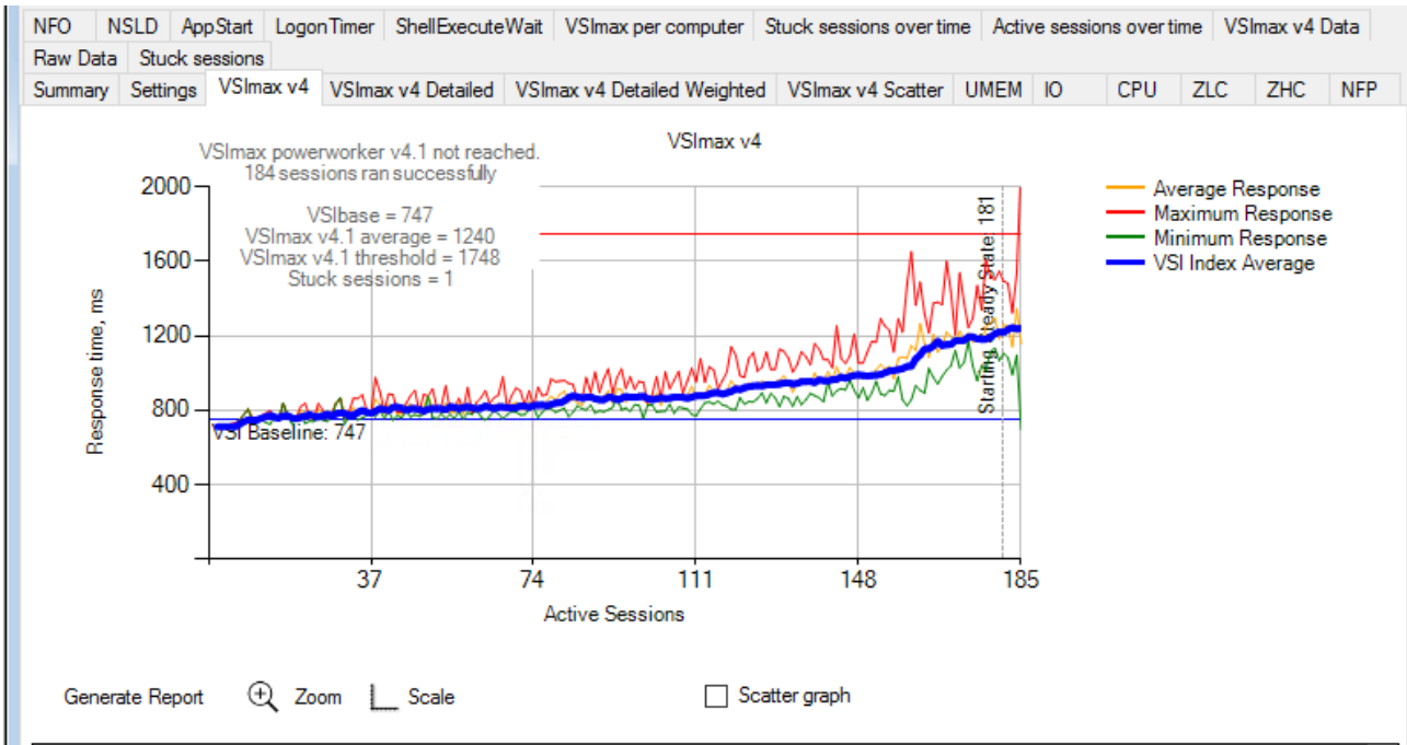
Figure 23. Login VSI end-user experience performance chart
