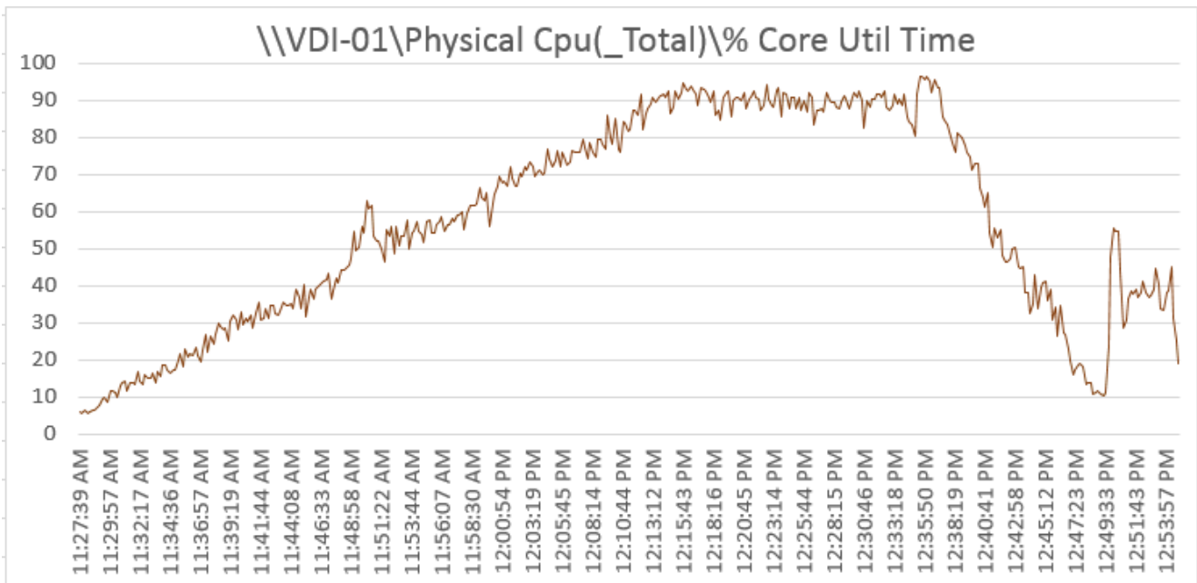
Figure 24. VMware ESX host CPU Util % during testing
