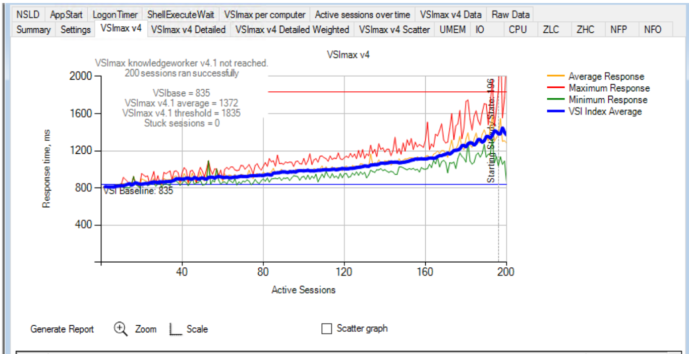
Figure 20. Login VSI end-user experience performance chart
