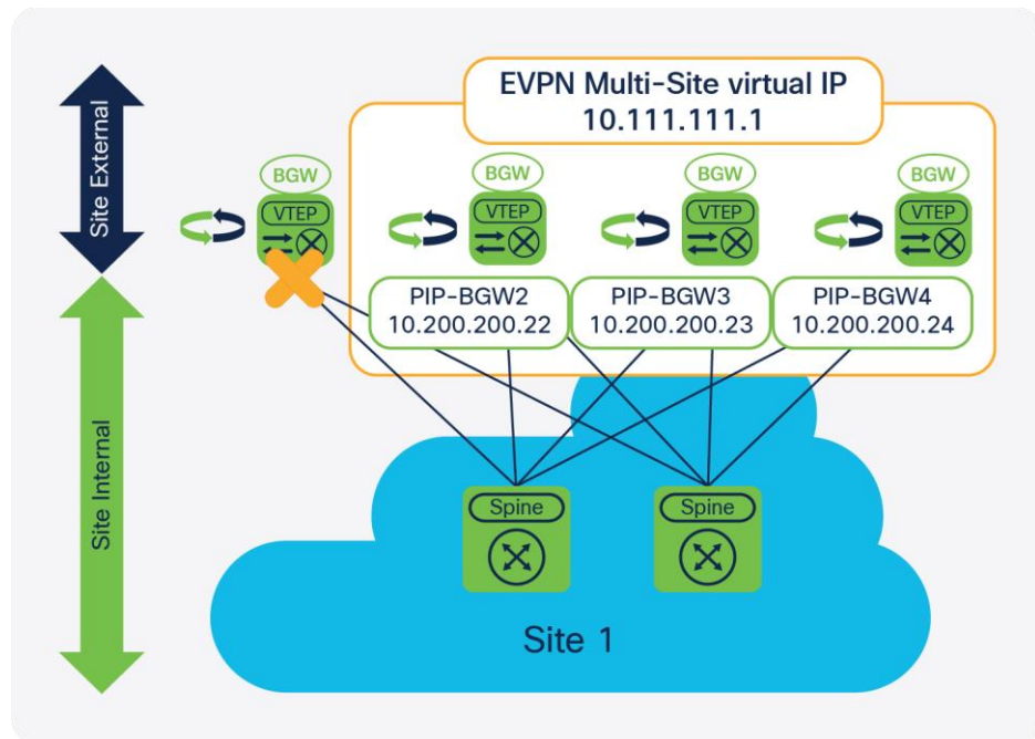
Figure 8. Fabric Isolation
