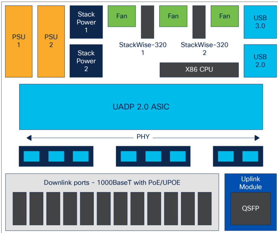
Figure 11. C9300LM-24U/48U/48T-4Y
