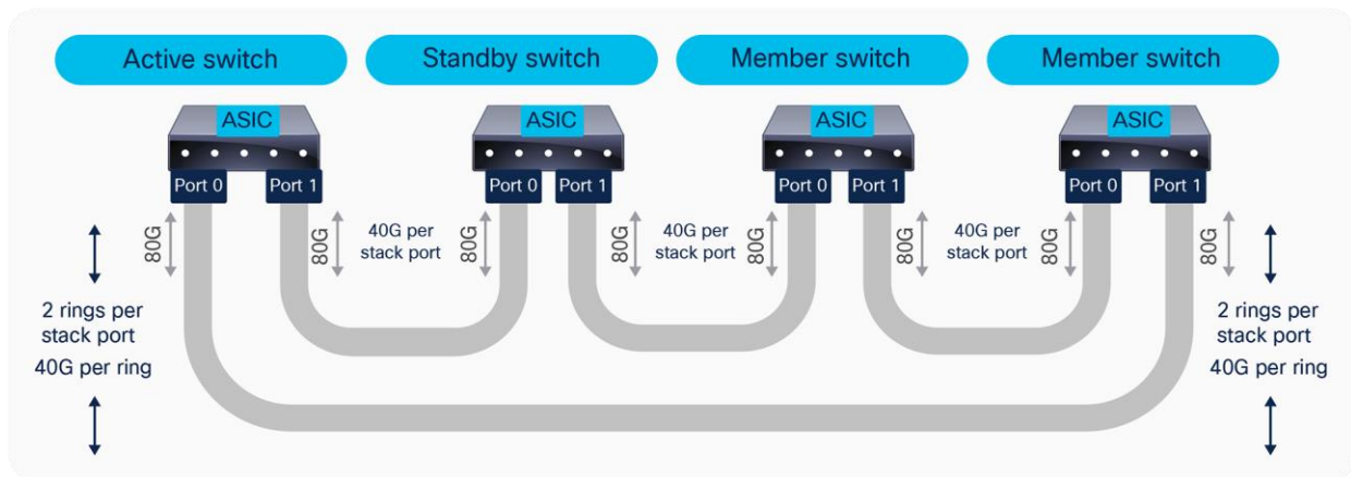
Figure 10. StackWise-160 architecture
