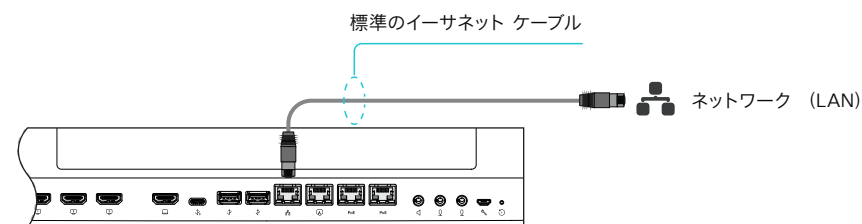
Room Bar Pro
