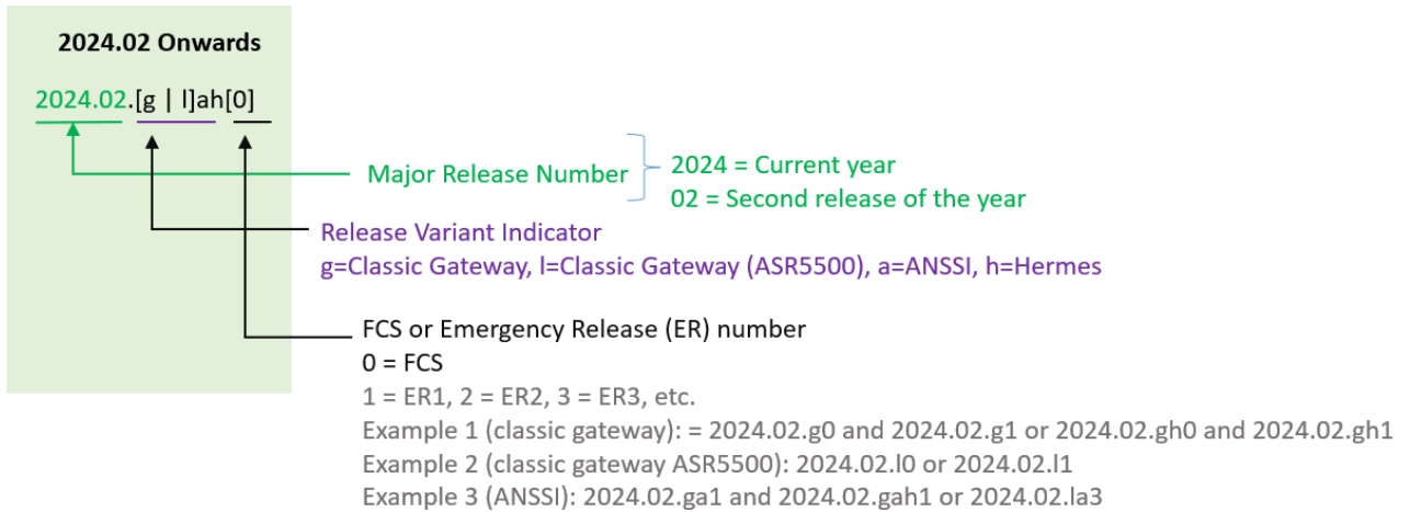
Figure 1 – Version Numbering
