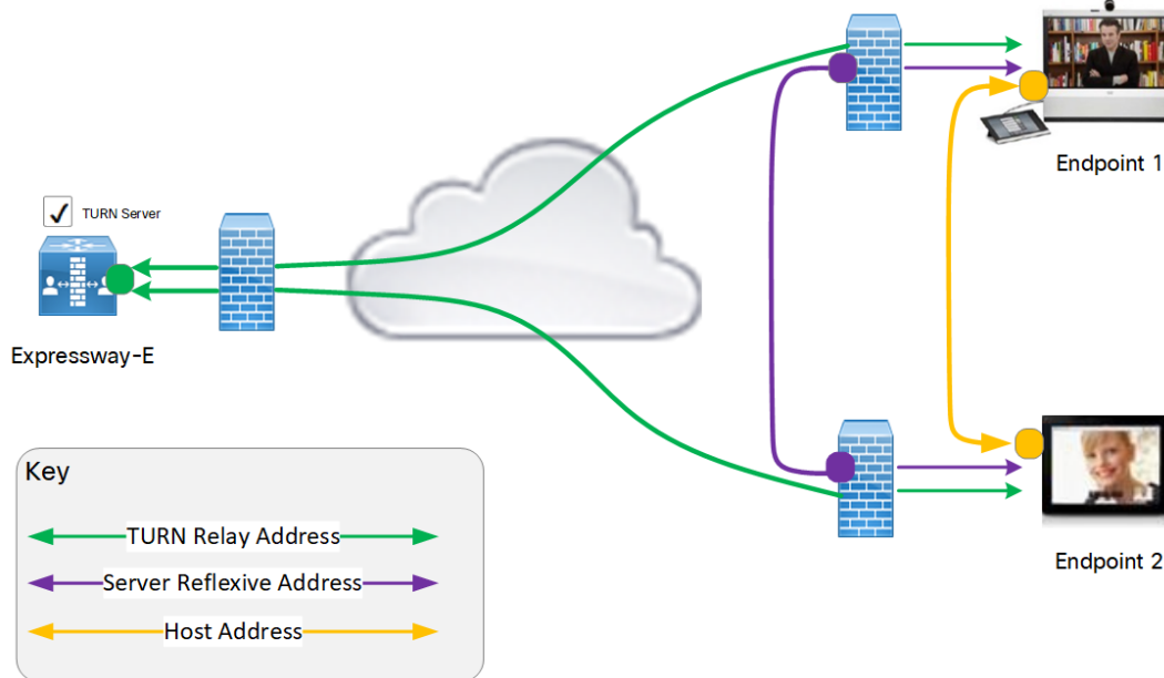
Figure 5 ICE Media connection paths
