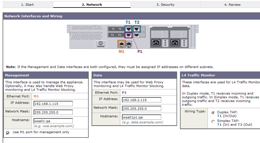
Figure 4-1 System Setup Wizard – Network Tab, Network Interfaces and Wiring Page
