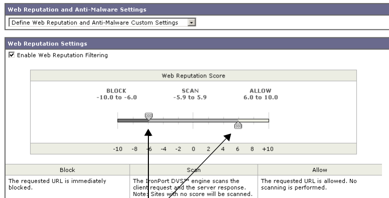
Figure 18-1 Web Reputation Filter Settings for Access Policies
