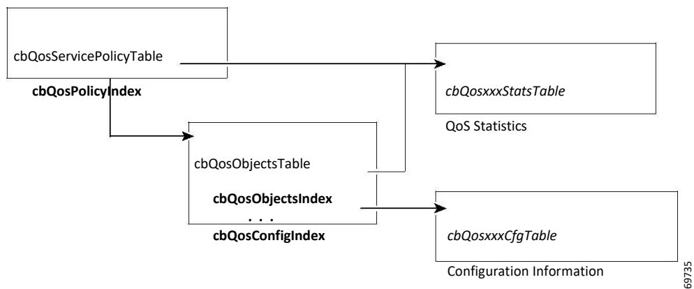
Figure 1-2 The Cisco ASR 9000 Series Router QoS Indexes
