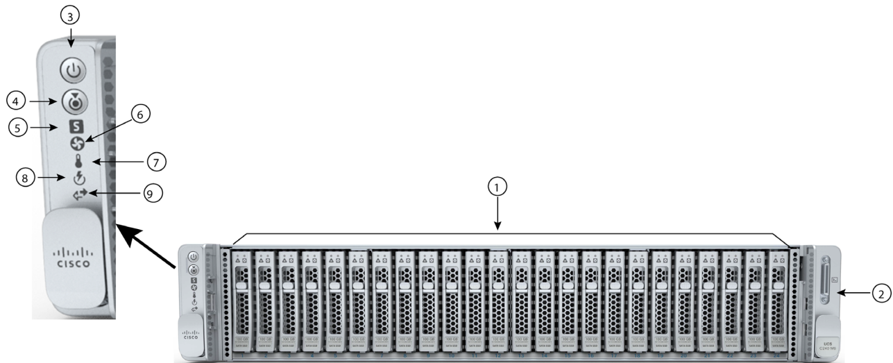
Figure 2 Chassis Front View: HXAF240C-M6SN-EXP (All NVMe)
